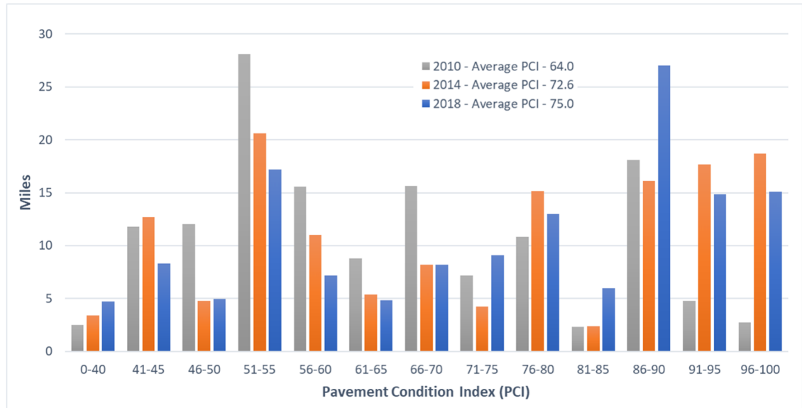
Figure 1 PCI Distribution Chart
